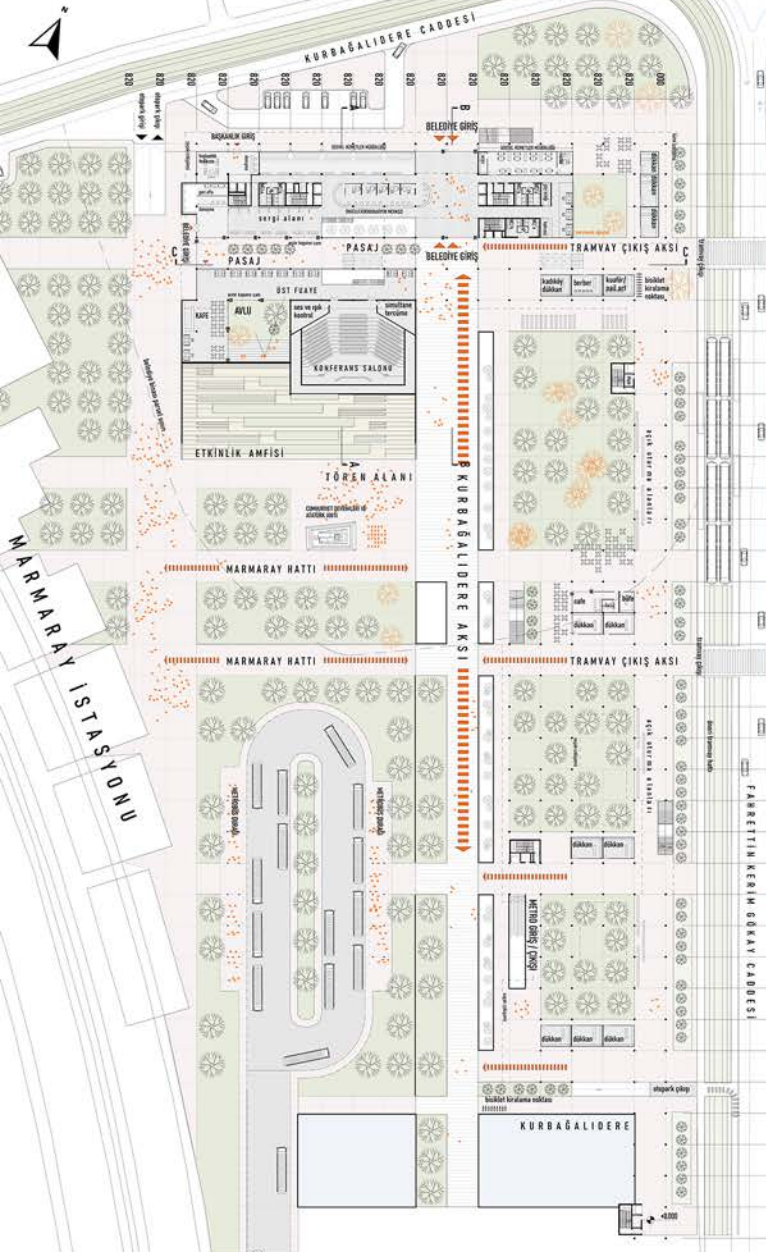
+00.00 KAT PLANI 0:1/500
